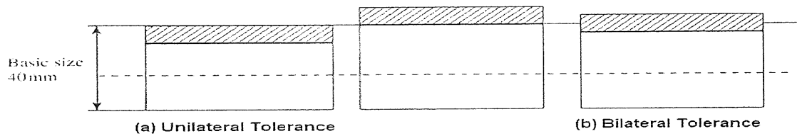
Figure 2: tolerance classification
