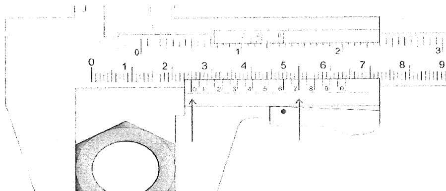
Figure 3: Vernier Caliper
