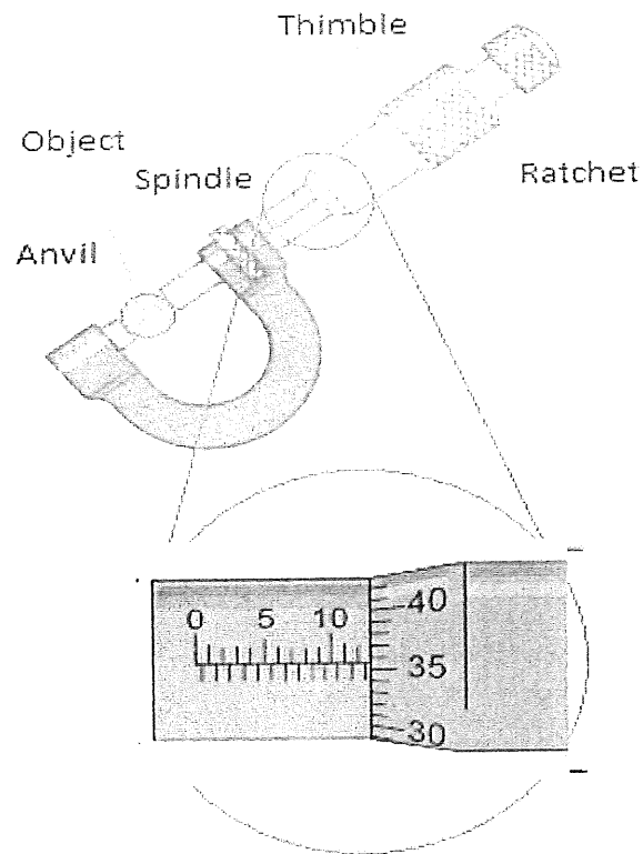
Figure 4: Micrometer
